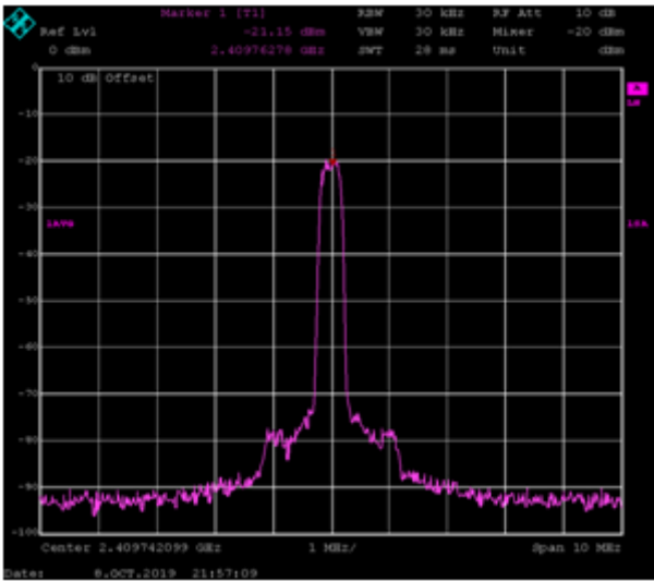
SPF5043 + 10dB Pad on o/p
