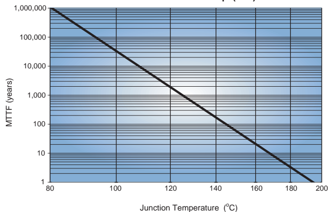
MTTF vs. Junction Temp. (Gali)
