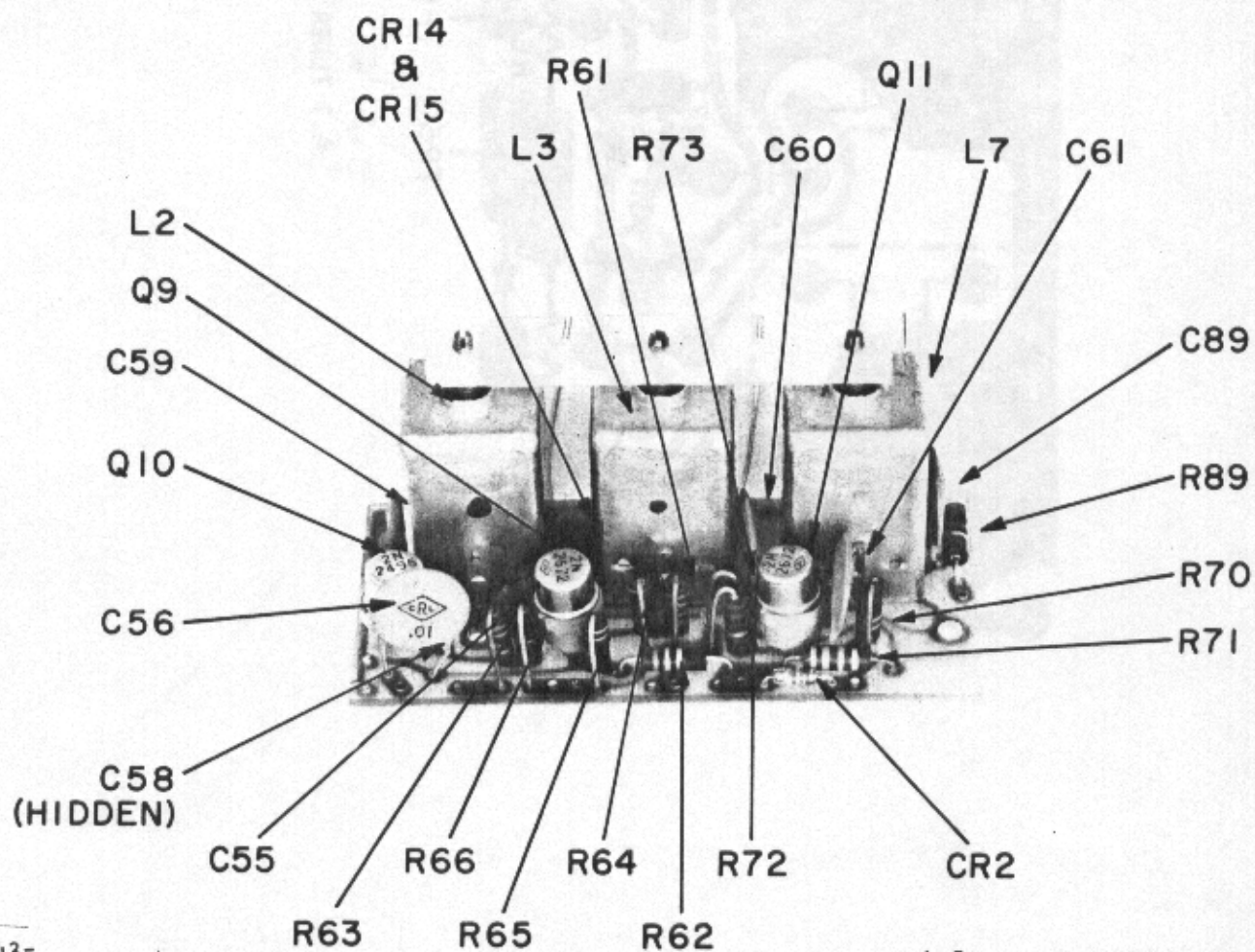
4.5 TUNER BOARD
